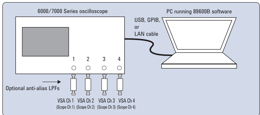
Figure 1c. Equipment connections for 4-channel oscilloscope used to provide 3- or 4-channel VSA measurements using the 89600B VSA software. 1
